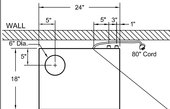
PLAN VIEW
